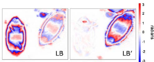
Figure 8. Horizontal linear birefringence (LB) and 45° linear birefringence (LB') as determined from the Mueller matrix measured at 500 nm for two crystallites with different orientations. The discontinuities in sign (sharp red to blue transitions) are due to changes in the order of birefringence.
