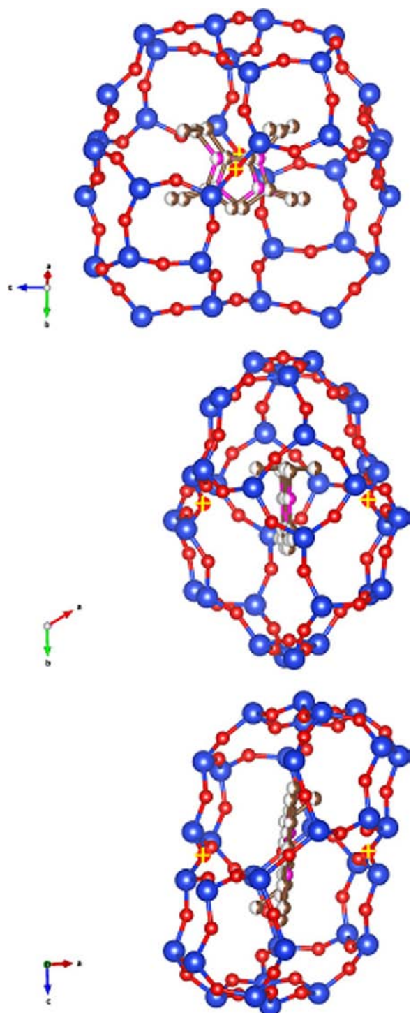
Figure 5. Three views along the directions specified by the arrows of the large [4^6 5^8 8^2 10^2] cavity of HPM-1, containing the 2E134TMI cation. Two symmetrical orientations of the cation are shown. In each view, two O(2) atoms defining the minimum thickness of the cavity across the imidazolium ring are marked with a yellow cross (blue, silicon; red, oxygen; white/brown, C; white/pink, N).
