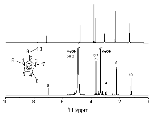
Figure 2. ^1\text{H} NMR spectra in \text{D}_2\text{O} solution of the dissolved 2E134TMI-STW zeolite (bottom) and of the pristine 2E134TMI iodide (top).
