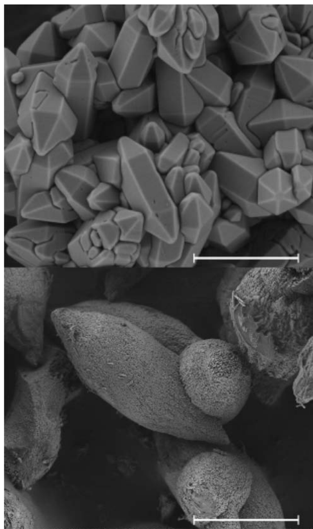
Figure 4. FE-SEM pictures of as-made HPM-1 showing two typical yet distinct morphologies: bipyramidal hexagonal rods (crystallized at H_2O/SiO_2 = 4 , for 5 days, top, scale bar 2 \mu m ) and podlike aggregates ( H_2O/SiO_2 = 5.5 , 16 days, bottom, scale bar 10 \mu m ). Both materials were synthesized at 175 ^{\circ}C .
