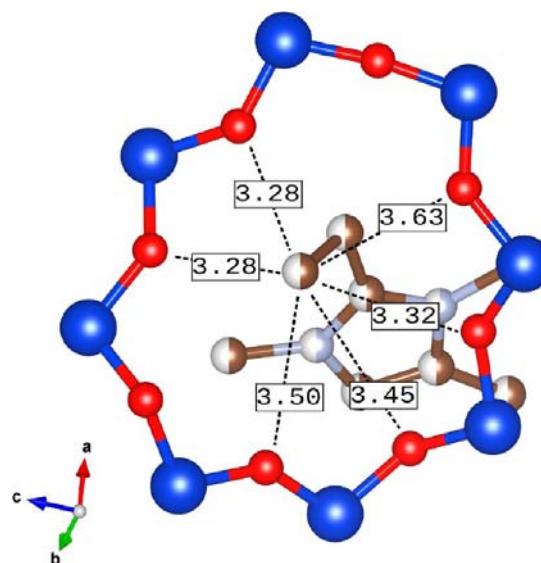
Figure 6. Closest O–C distances (Å) between the O of the 8MR window and the -\text{CH}_3 end of the ethyl substituent of 2E134TMI.
