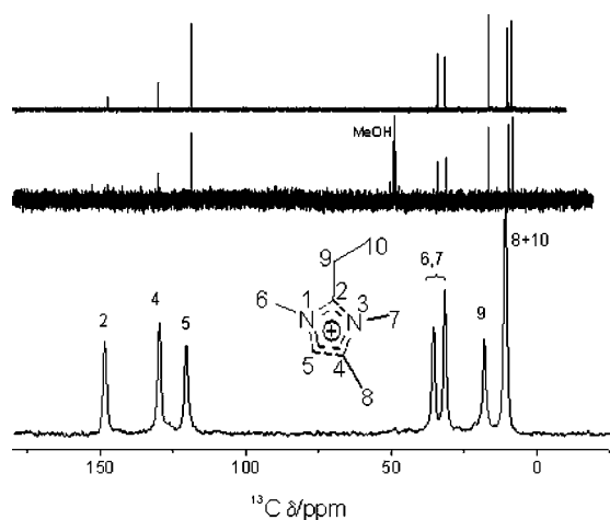
Figure 1. Solid-state ^{13}\text{C} MAS NMR spectrum of as-made 2E134TMI-STW (bottom) and ^{13}\text{C} NMR spectra in \text{D}_2\text{O} solution of the dissolved zeolite (middle; see the text, methanol added as a chemical shift reference) and of the pristine 2E134TMI iodide (top).
