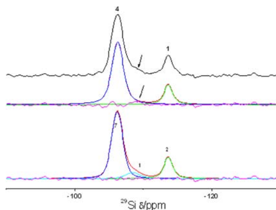
Figure 3. ^{29}\text{Si} MAS NMR spectrum of as-made 2E134TMI-STW (top). Two deconvolutions with two or three resonances are shown (with relative intensities of the deconvoluted components as indicated). The simulations also show a difference spectrum.
