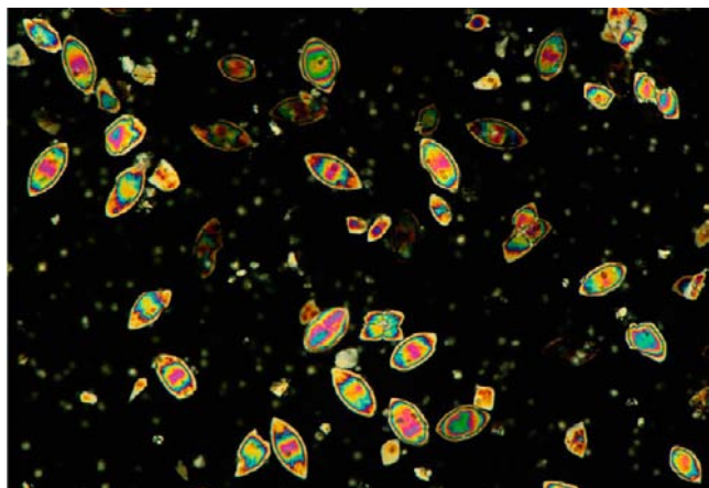
Figure 7. HPM-1 zeolite dispersed in index-matching oil and examined in a microscope under crossed polarizers (smaller crystallites correspond to zeolite ITW).
